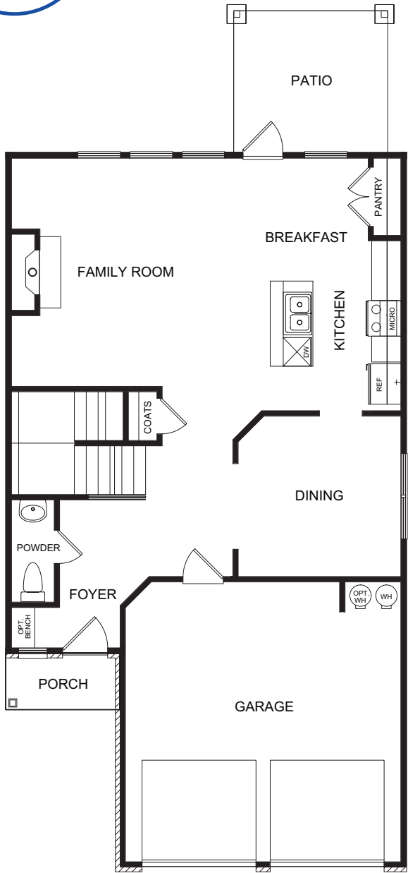
FIRST FLOOR
