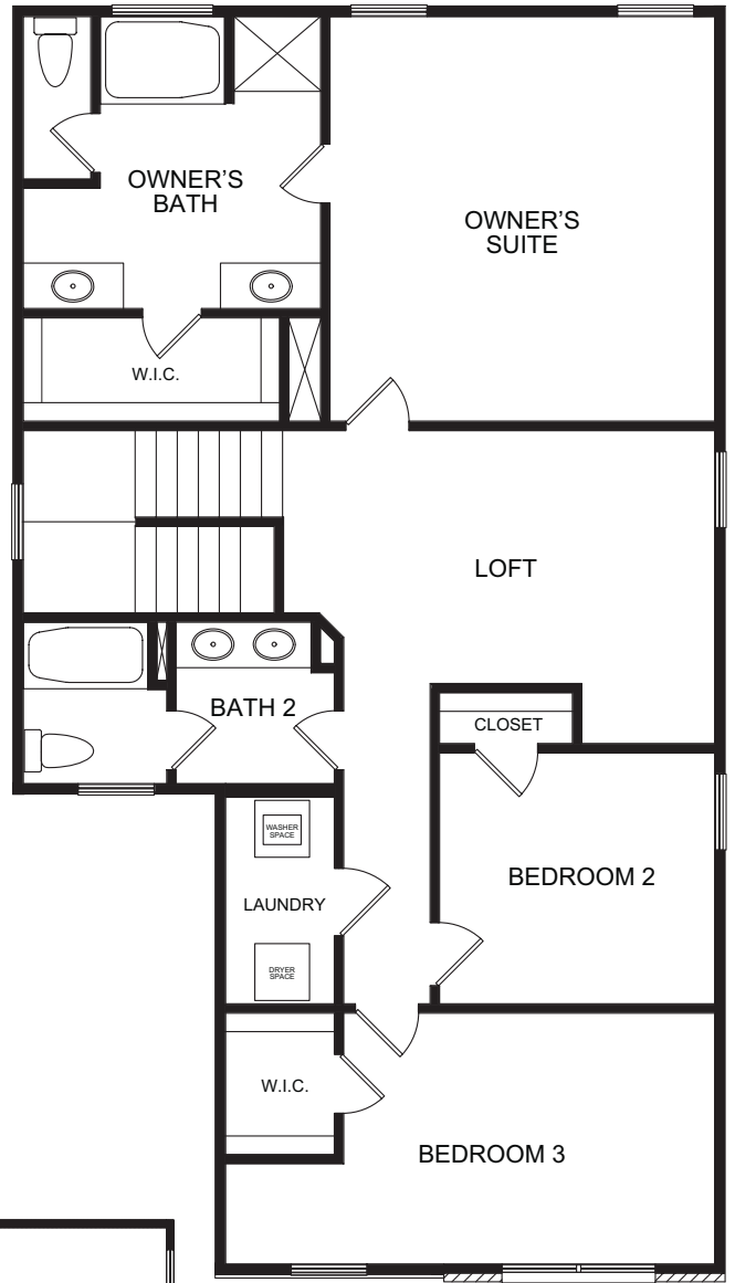
SECOND FLOOR
