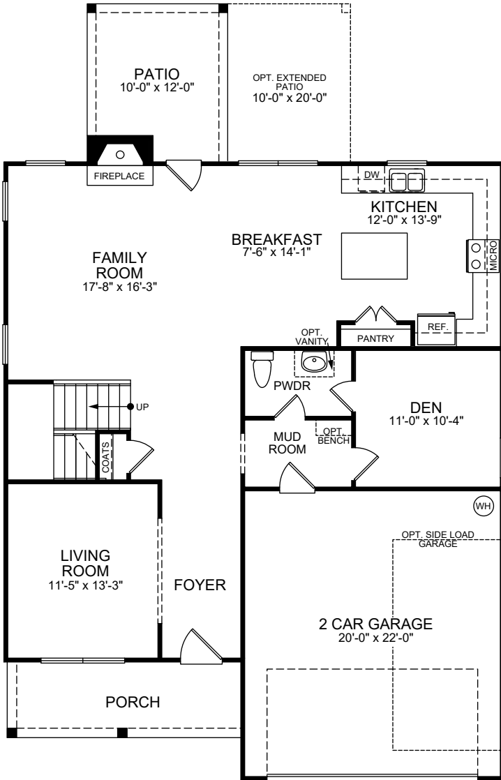
FIRST FLOOR
