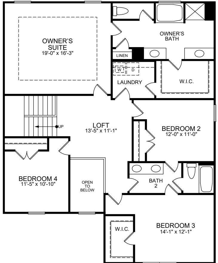
SECOND FLOOR
